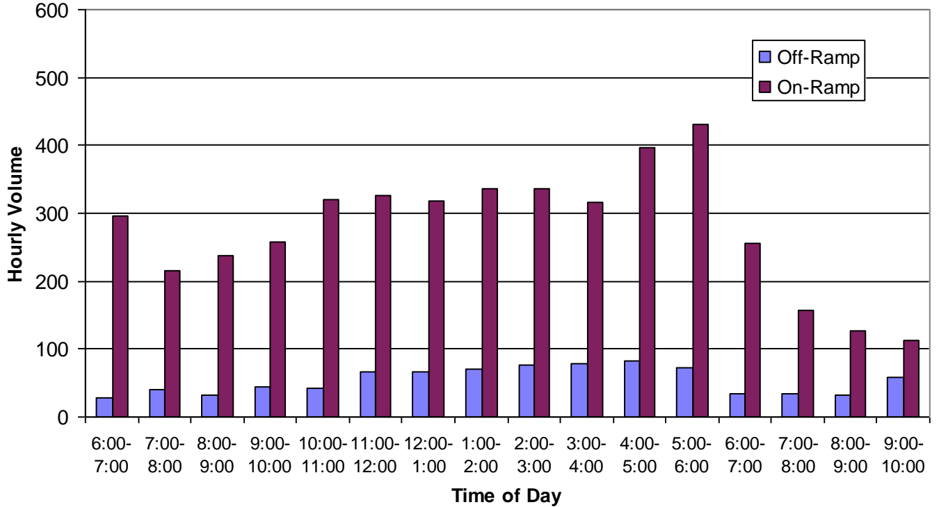
Exhibit 12.3-3 Daily Traffic Volume Profile for I-82 Northbound Ramps at US 730
