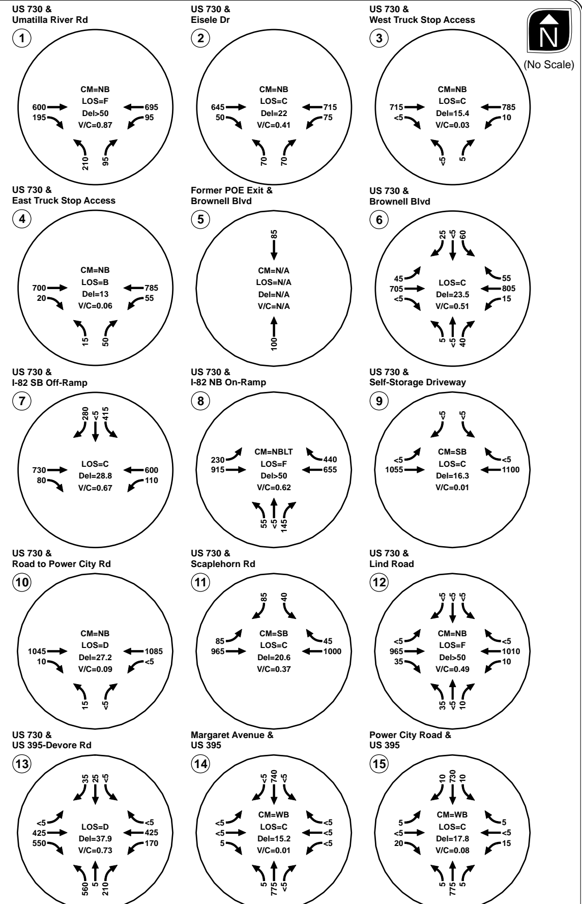
YEAR 2030 CONCEPT 13 OPERATIONS 30TH HIGHEST HOUR - EXISTING POE SITE VACANT UMATILLA, OREGON
