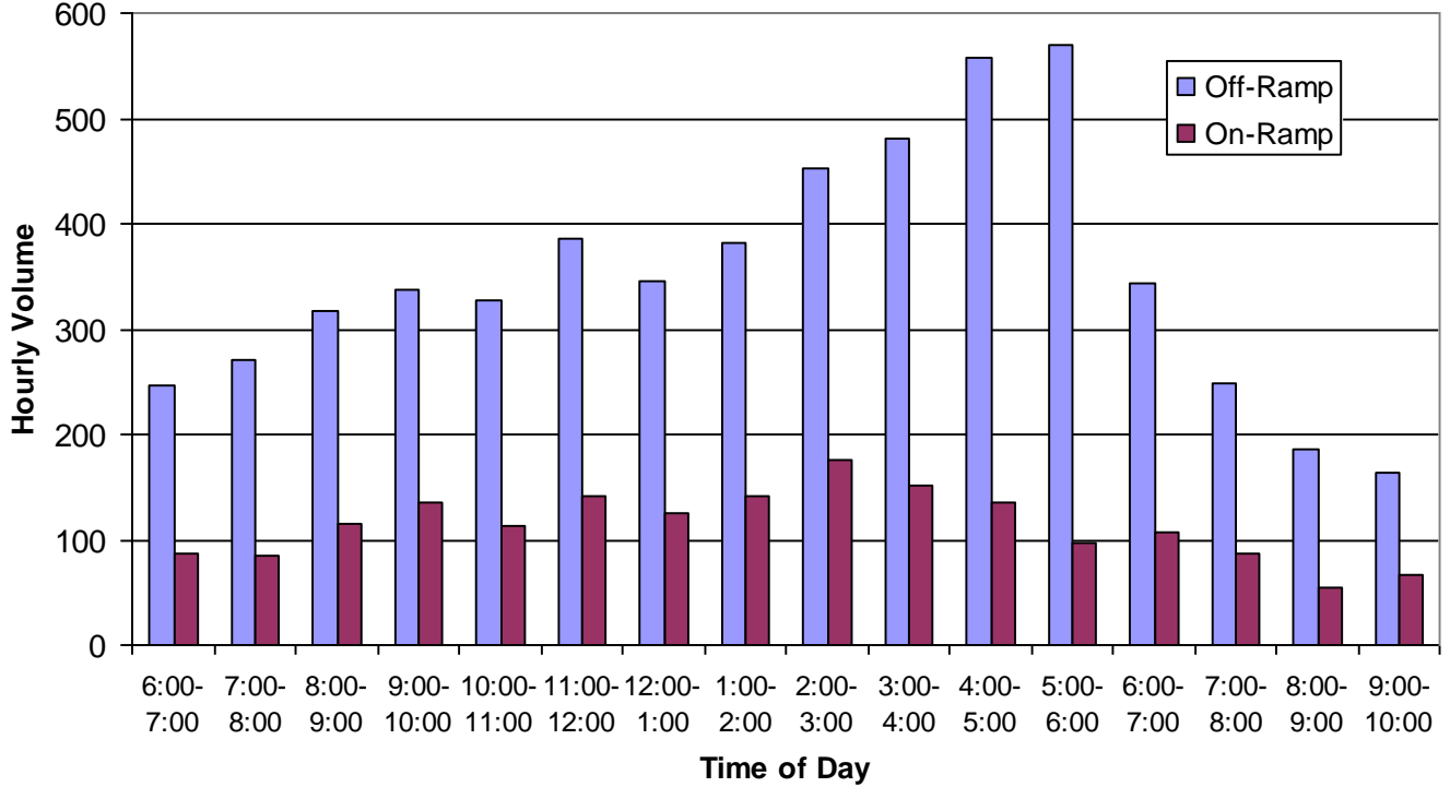
Exhibit 12.3-2 Daily Traffic Volume Profile for I-82 Southbound Ramps at US 730
