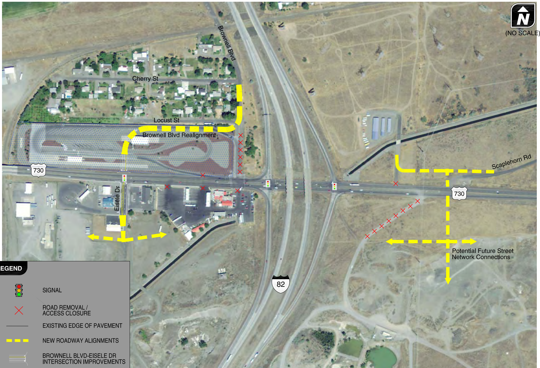
CONCEPT 13 I-82/US 730 INTERCHANGE AREA UMATILLA, OREGON
