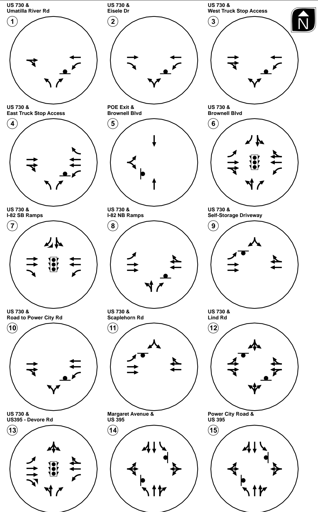
EXISTING LANE CONFIGURATIONS AND TRAFFIC CONTROL DEVICES UMATILLA, OREGON FIGURE
