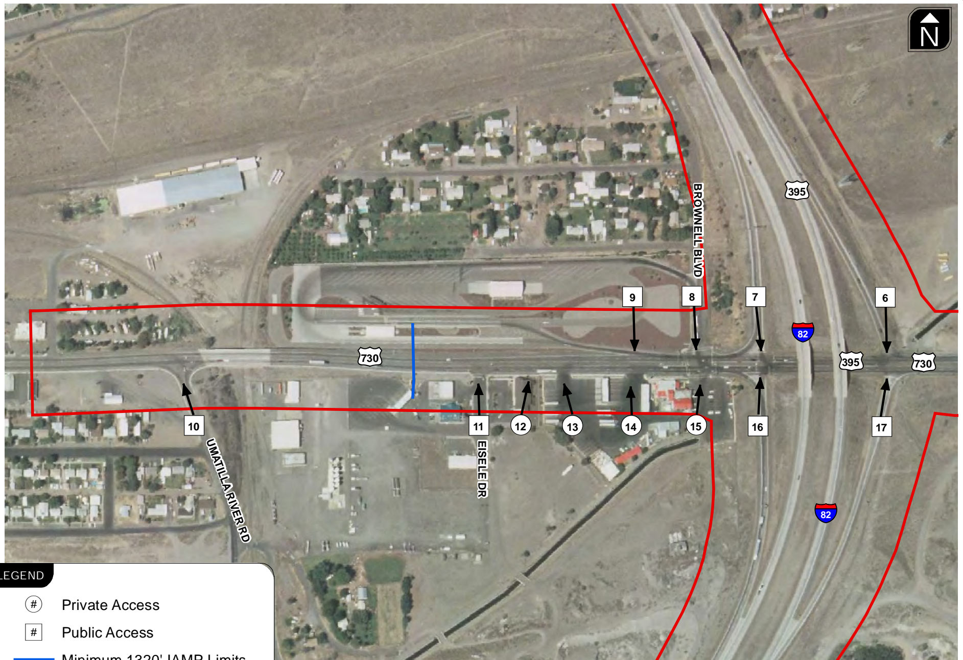
ACCESS INVENTORY WEST OF I-82 AND I-82 RAMPS UMATILLA, OREGON FIGURE
